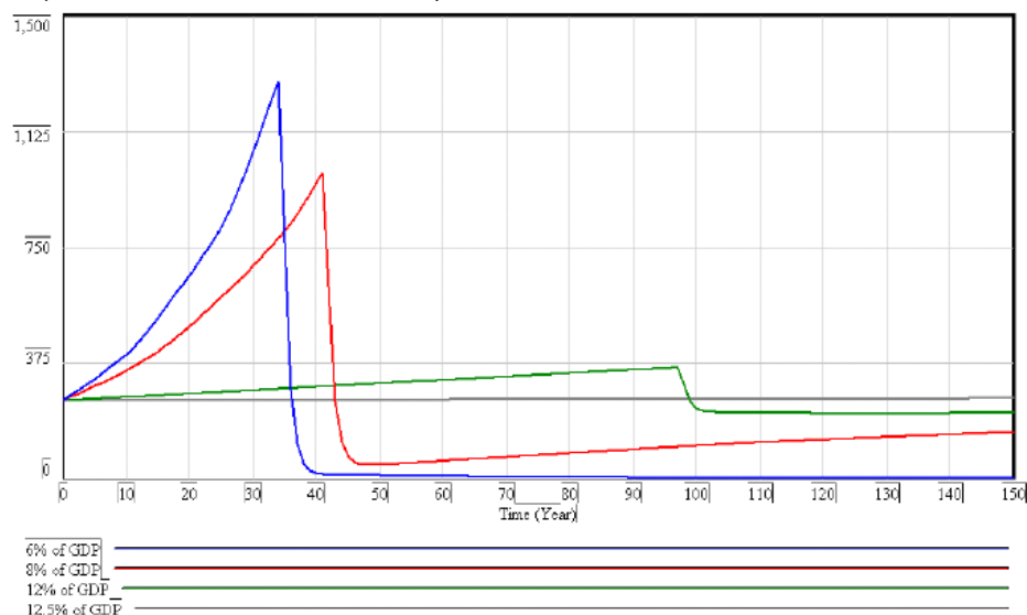
Consumption paths for different levels of investment in alternative energy (high initial capital level).
