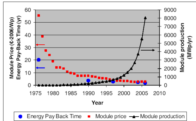
Figure 1: Historical development of module prices (squares, left y-axis, €-2006/Wp), production volumes (triangles, right y-axis, MWp/yr) and Energy Pay-Back Time (circles, left y-axis, yr). Sources: refs. [1-8]
