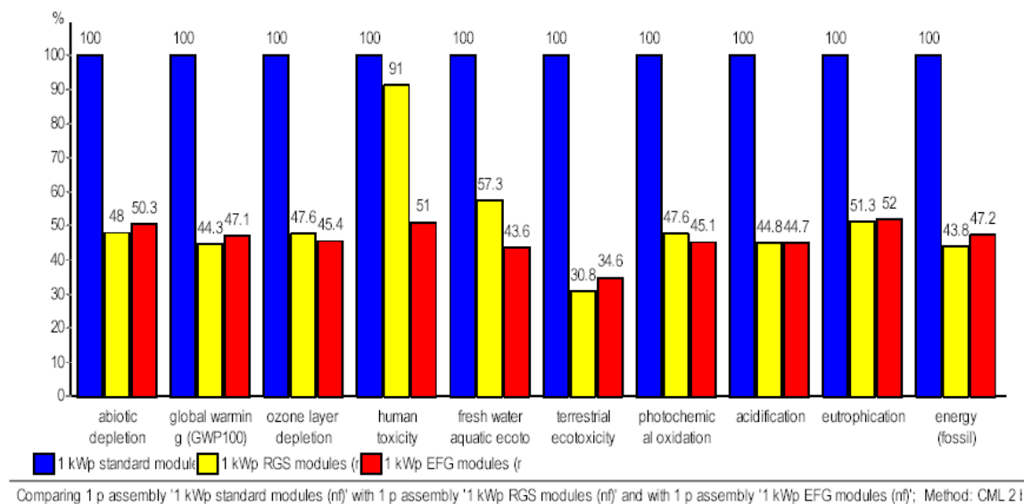
Figure 1: Comparison of LCA results for 1 kWp of PV modules on the basis of three investigated production technologies, namely standard-2000, Solsilc/RGS and Bayer/EFG.
